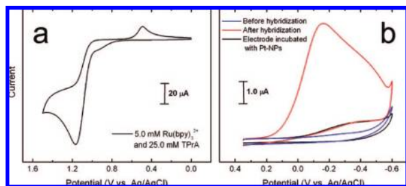
Figure 2. Cyclic voltammograms obtained from a macroscopic gold working electrode configured within a standard three-electrode cell. (a) The solution contained 5.0 mM Ru(bpy) 3 2+ and 25.0 mM TPrA in 0.100 M phosphate buffer. (b) The solution contained air-saturated 0.100 M phosphate buffer, and the CVs were obtained after modification of the electrode with probe DNA (blue), after hybridization with Pt-NP-labeled cDNA (red), and after incubation of a probe-modified electrode with a 100 nM solution of free Pt-NPs (no cDNA, black CV). Scan rate: 100 mV/s.
